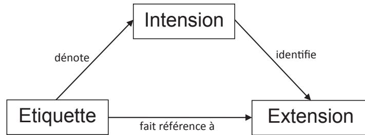
FIGURE 2.1: Triangle sémiotique.
