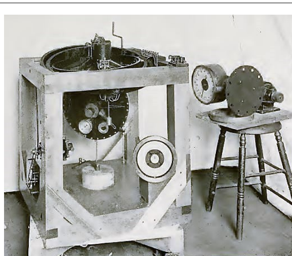
Illustration 47 : Gyroscop SPERRY
