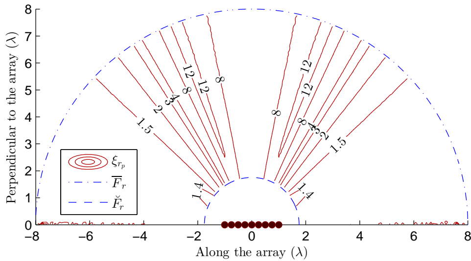
Figure B.5 – \check{\zeta}_{r_p} of [2], corrected using section 3.3; d = \lambda/4 , L = 10^3 , and \check{N} = 4 .
