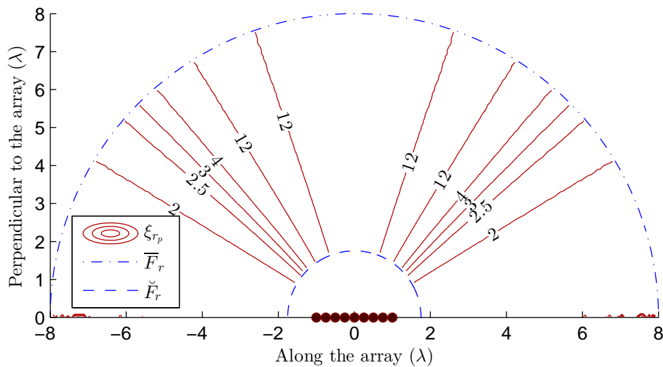
Figure B.6 – \check{\zeta}_{r_p} of [3], corrected using section 3.3; d = \lambda/4 , L = 10^3 , and \check{N} = 4 .
