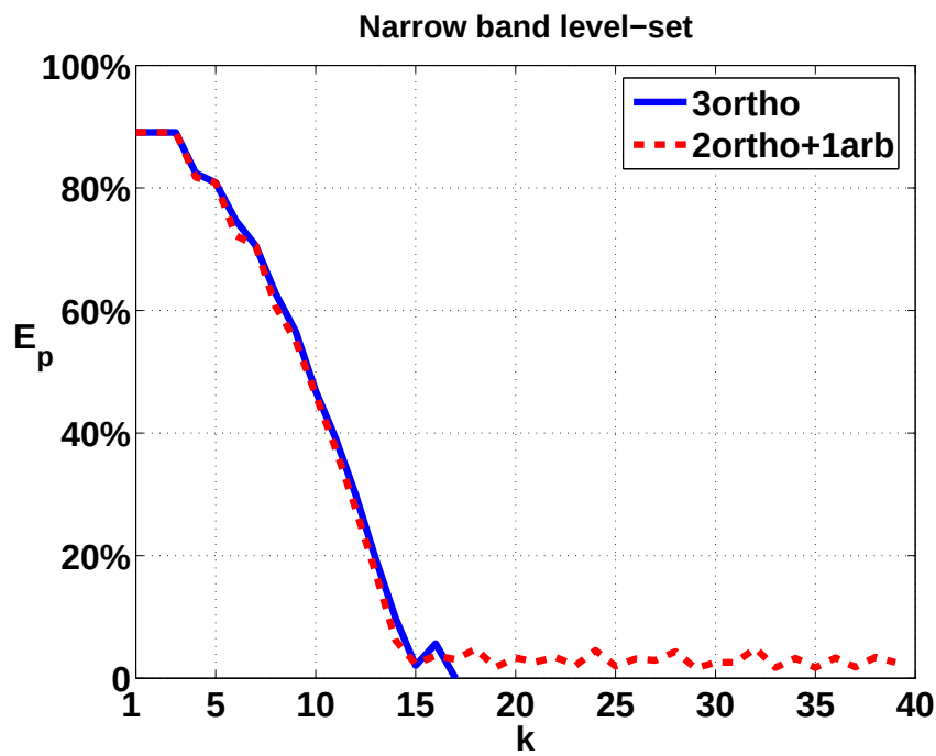
Figure 3.39: Comparison between the '3ortho' and '2ortho+1arb' cases for the sphere reconstruction with the 'Narrow band' method for: (a) the normalized residual r_k with respect to the iteration k ; (b) error in pixels E_p comparing to the original object.
