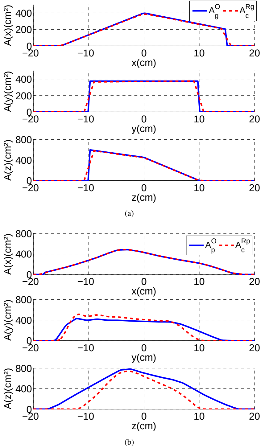
Figure 3.6: Quality evaluation of 3D image reconstruction in Fig. 2.12: (a) Comparison between the analytical geometrical profile functions A_g^O of the initial object and the profile functions A_c^{Rg} computed from its reconstructed object Rg ; (b) Comparison between the physical profile functions A_p^O of the initial object and the profile functions A_c^{Rp} computed from its reconstructed object Rp , in direction x, y, z, respectively.
