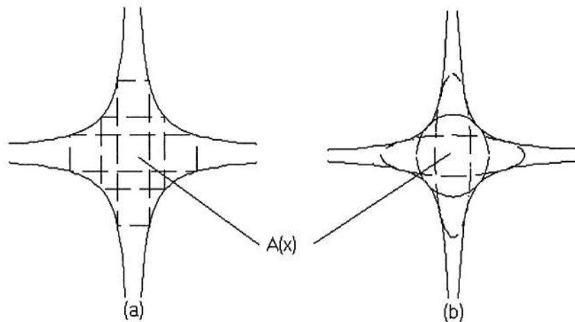
Figure 2.8: hyperbolic contour: (a) K = 4 ; (b) K = 2\pi [5]
