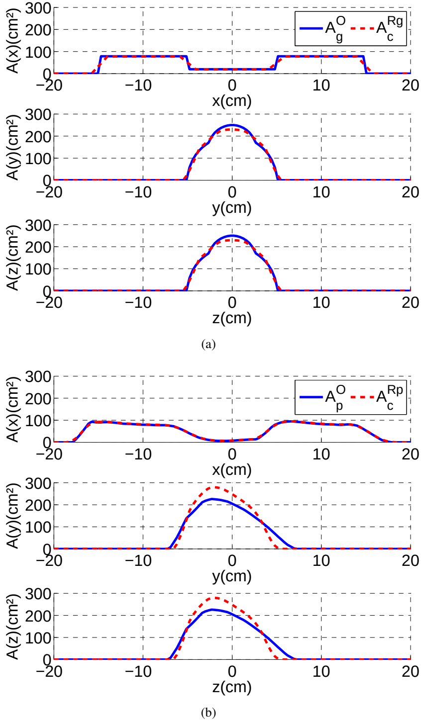
Figure 3.8: Quality evaluation of 3D image reconstruction in Fig. 2.14: (a) Comparison between the analytical geometrical profile functions A_g^O of the initial object and the profile functions A_c^{Rg} computed from its reconstructed object Rg ; (b) Comparison between the physical profile functions A_p^O of the initial object and the profile functions A_c^{Rp} computed from its reconstructed object Rp , in direction x , y , z , respectively.
