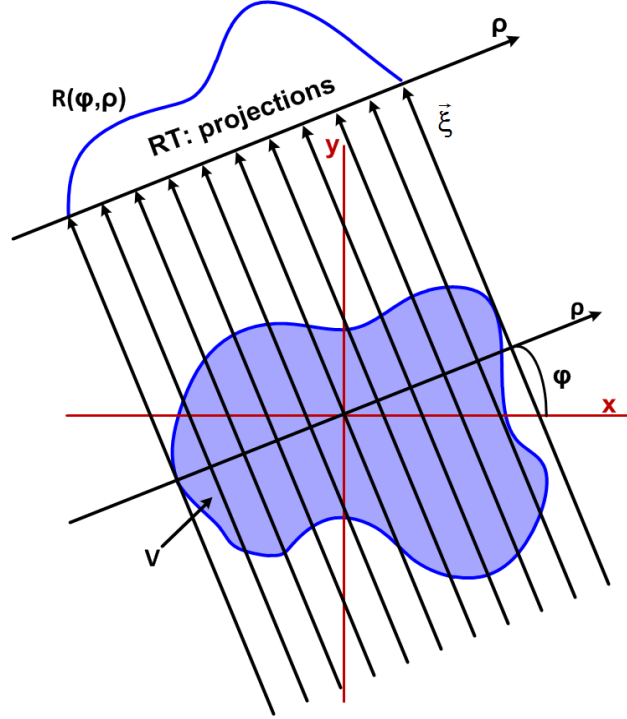
Figure 2.9: Geometric interpretation of the Radon transform.
