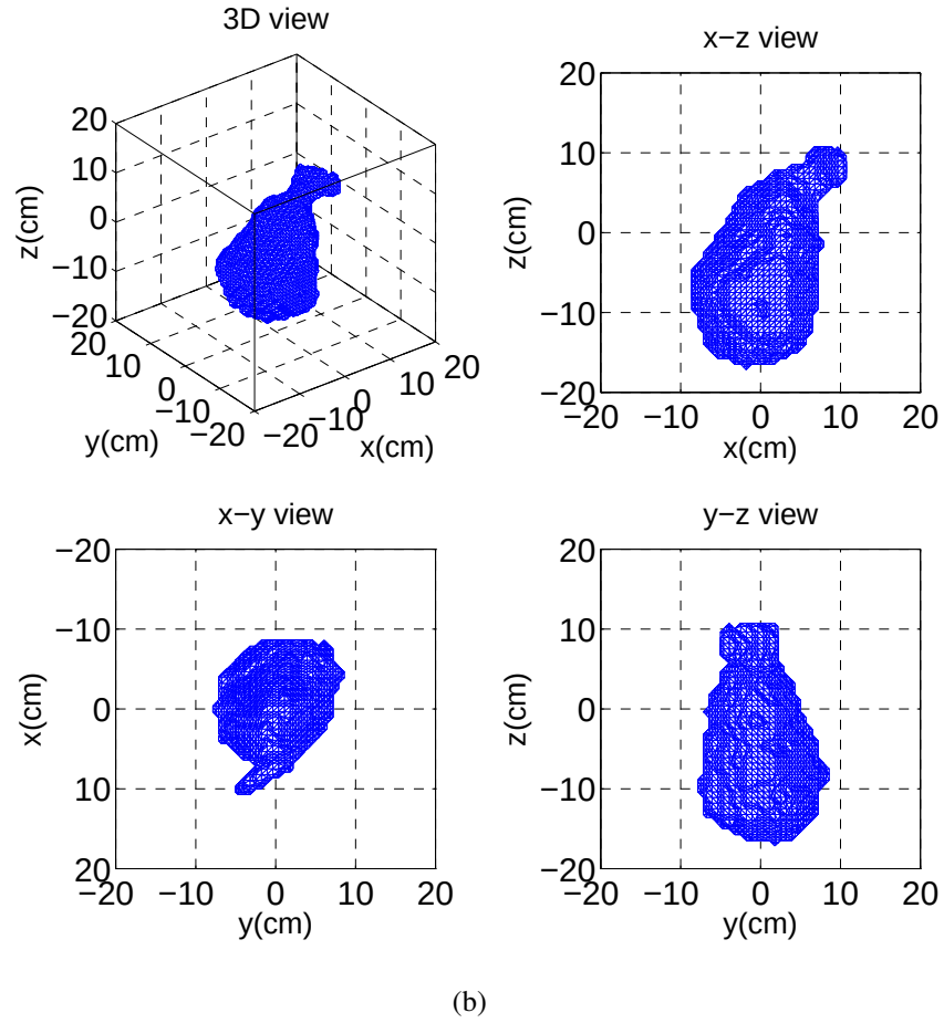
Figure 3.56: Configuration of study for the step-cylinder (Fig. 3.42) in the '3arb' case: (a) original geometrical profile functions; (b) reconstructed image obtained using the narrow band method at iteration k = 80 with error in pixels E_p = 45.3\% .
