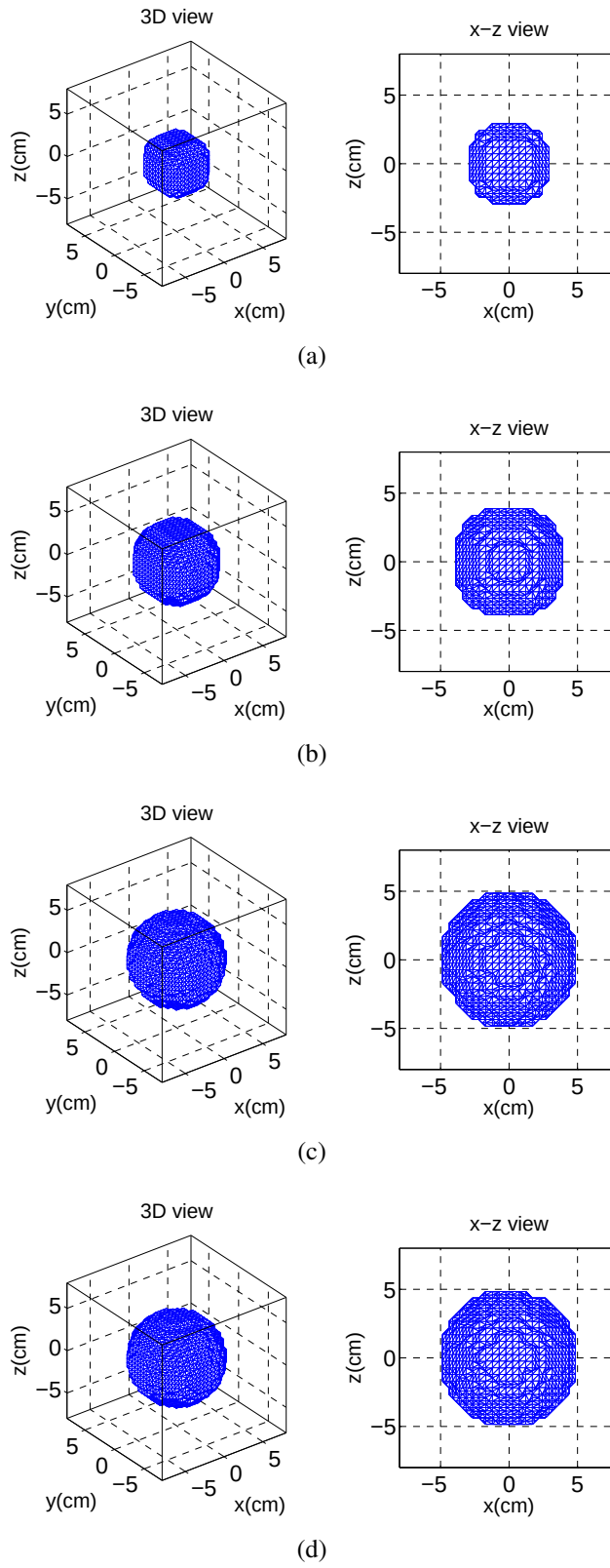
Figure 3.25: Evolution of the reconstructed 3D object in the '3ortho' case at iterations: (a) k = 5 ; (b) k = 10 ; (c) k = 15 ; (d) k_{final} = 19 .
