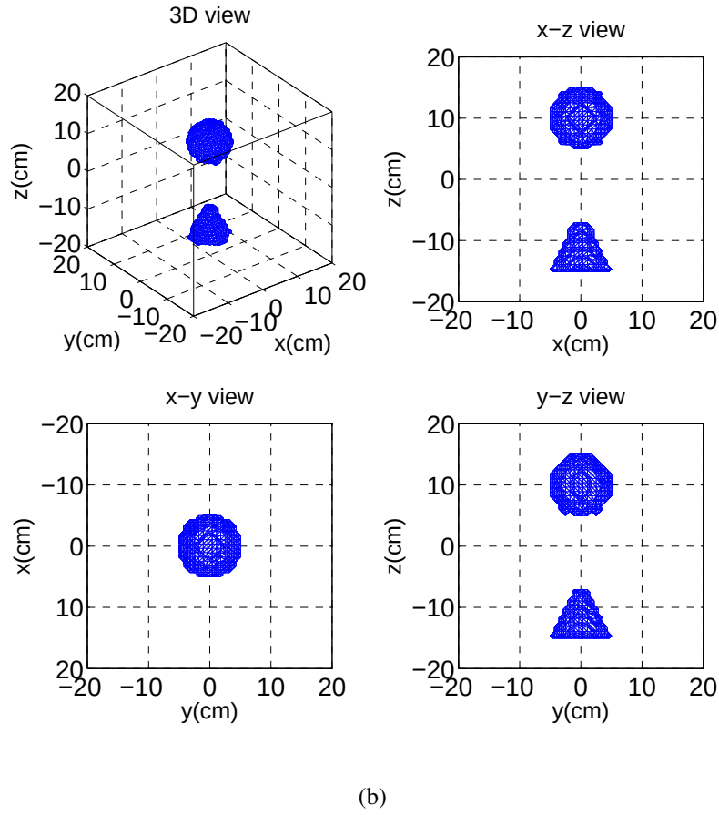
Figure 3.49: Configuration of study for the separated objects (Fig. 3.44) in the '3ortho' case: (a) original geometrical profile functions; (b) reconstructed image obtained using the narrow band method at iteration k = 80 with error in pixels E_p = 4.4\% .
