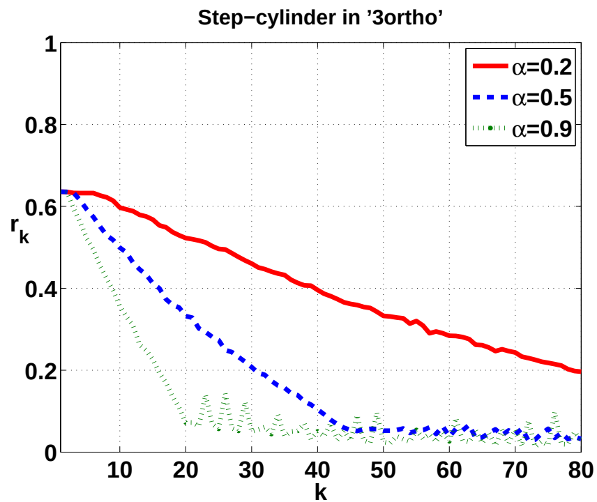
Figure 3.64: Effect of the time step \Delta t on the normalized residual r_k of the reconstruction with geometrical profile functions using the narrow band level set method for: (a) the sphere, (b) the step-cylinder, in the '3ortho' case.
