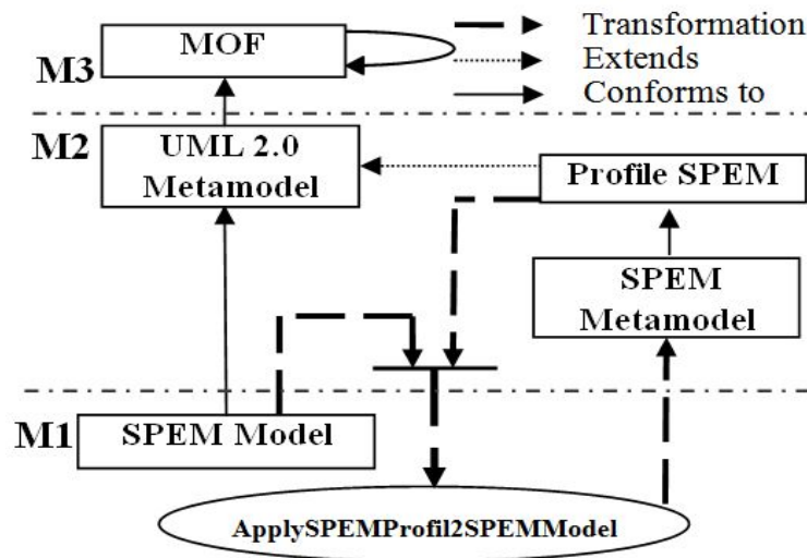
Figure 5.3 – Le module de transformation ATL ApplySPemProfil2SPemModel.
